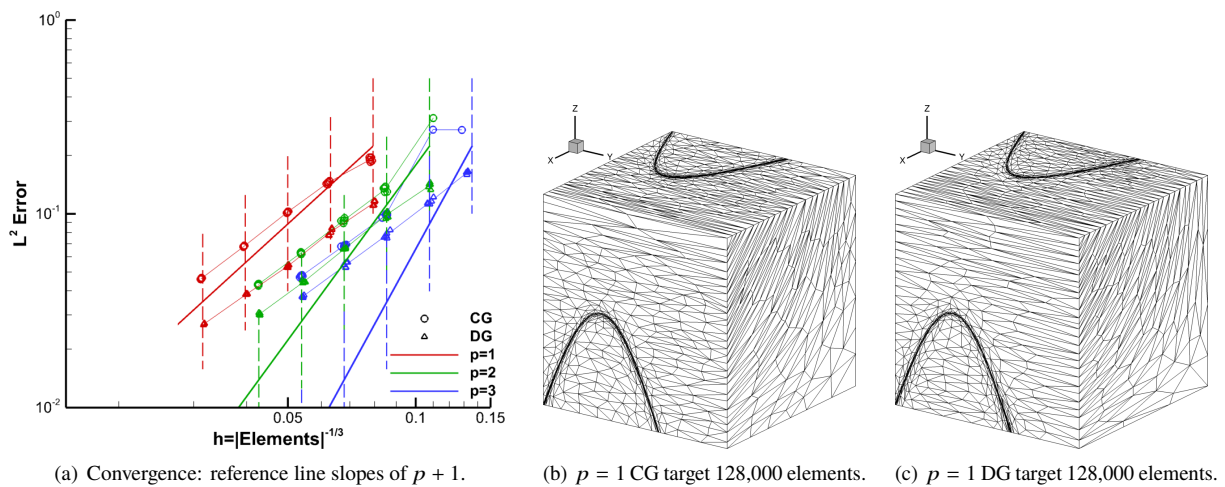
Fig. 54 sinatan3 L^2 -error MOESS convergence and grids using EPIC-ICSM.
