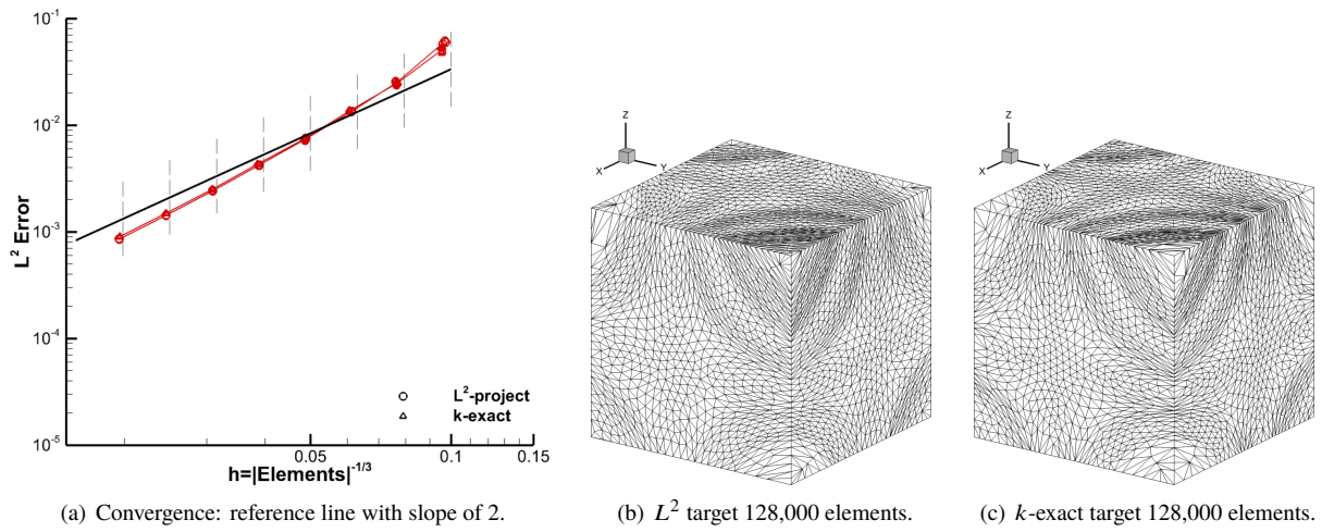
Fig. 32 sinfun3 L^2 -error multiscale metric convergence and grids using avro.
