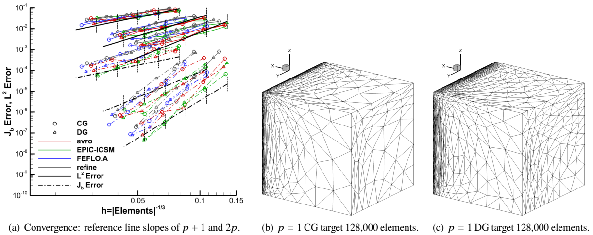
Fig. 19 TripleBL L^2 -error and J_b -error MOESS convergence. Example meshes adapted with FEFLO.A.
