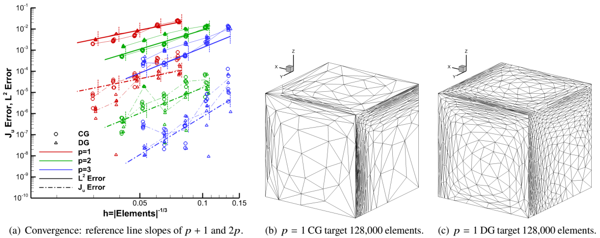
Fig. 63 TripleBL L^2 - and \mathcal{J}_u -error MOESS convergence and grids using avro.
