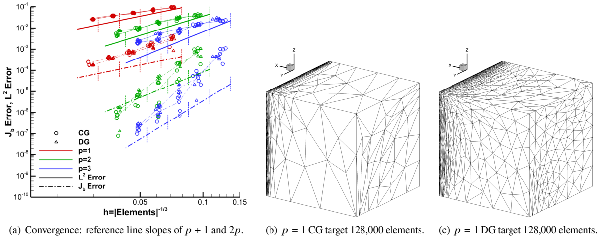
Fig. 64 TripleBL L^2 - and \mathcal{J}_b -error MOESS convergence and grids using refine.
