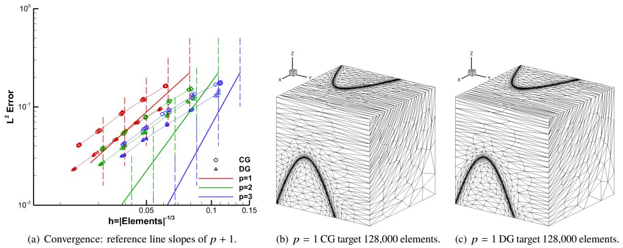
Fig. 53 sinatan3 L^2 -error MOESS convergence and grids using FEFLO.A.
