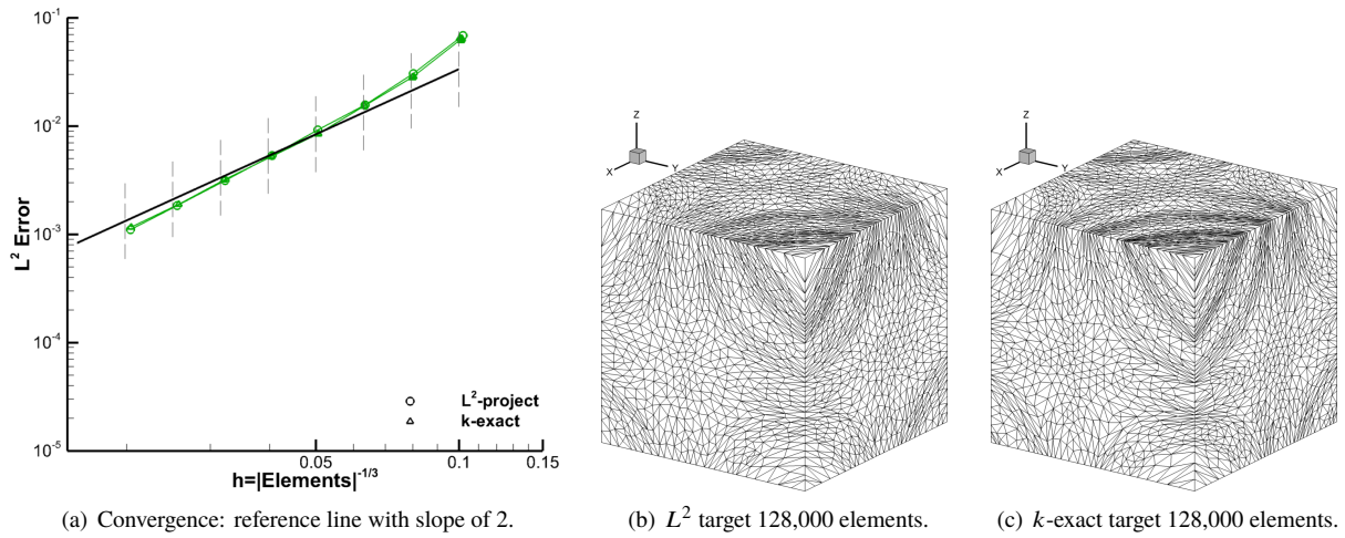
Fig. 31 sinfun3 L^2 -error multiscale metric convergence and grids using EPIC-ICSM.
