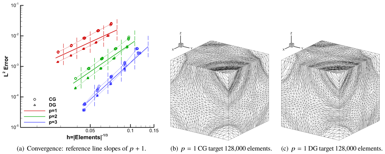
Fig. 35 \text{sinfun3} L^2 -error MOESS convergence and grids using FEFLO.A.
