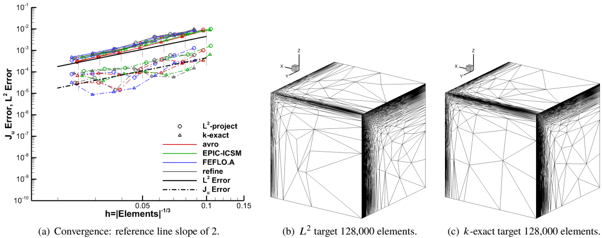
Fig. 16 L^2 -error and \mathcal{J}_u -error multiscale metric convergence. Example meshes adapted with refine.
