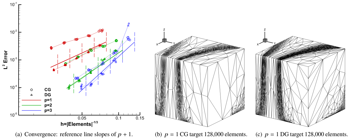
Fig. 43 \tanh 3 L^2 -error MOESS convergence and grids using refine.
