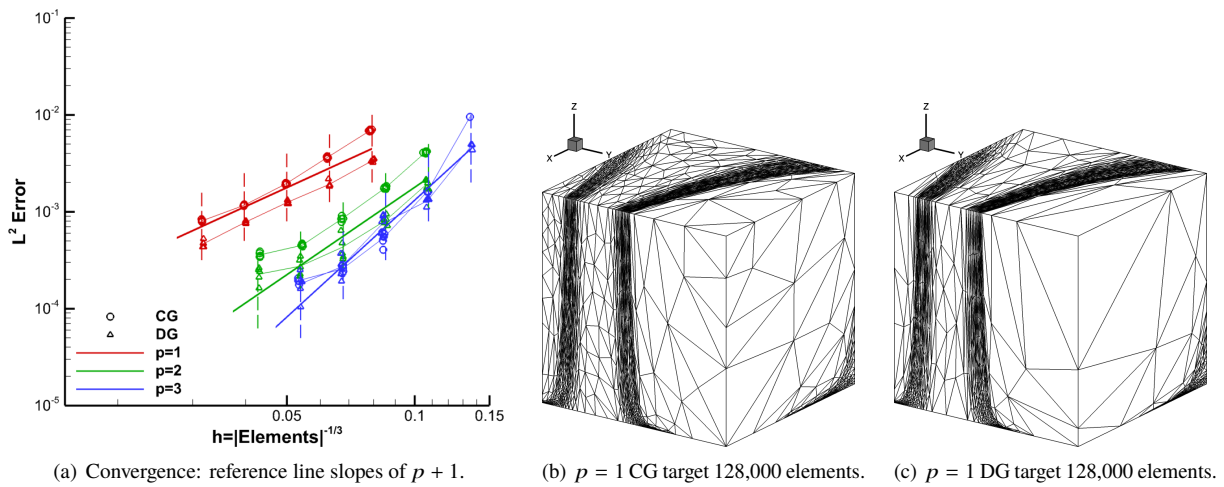
Fig. 45 \tanh 3 L^2 -error MOESS convergence and grids using EPIC-ICSM.
