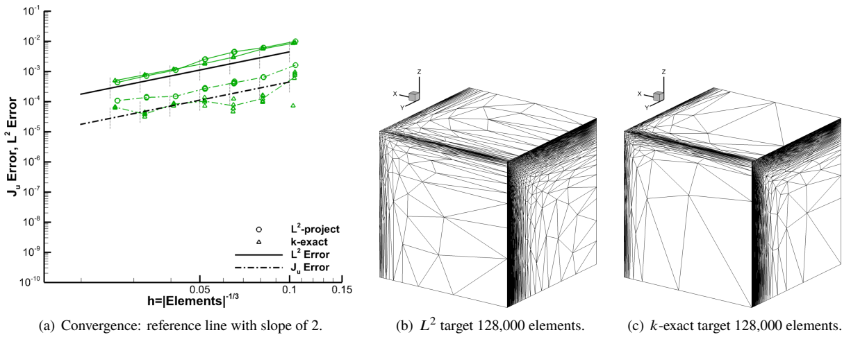
Fig. 58 TripleBL L^2 -error multiscale metric convergence and grids using EPIC-ICSM.
