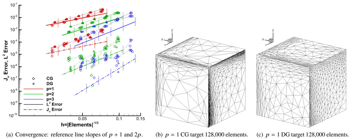
Fig. 60 TripleBL L^2 - and J_u -error MOESS convergence and grids using refine.
