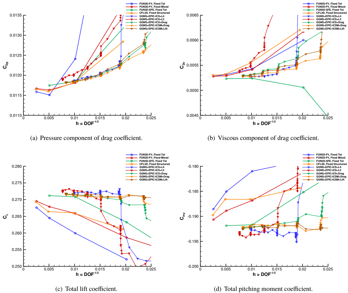
Fig. 68 ONERA M6 force and moment convergence, GGNS+EPIC.
