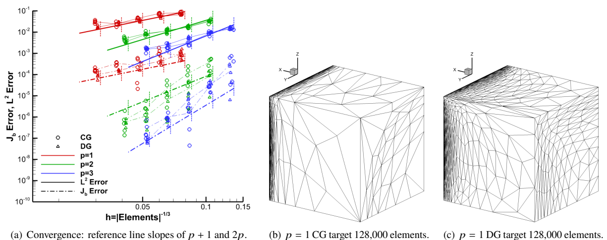
Fig. 67 TripleBL L^2 - and \mathcal{J}_b -error MOESS convergence and grids using avro.
