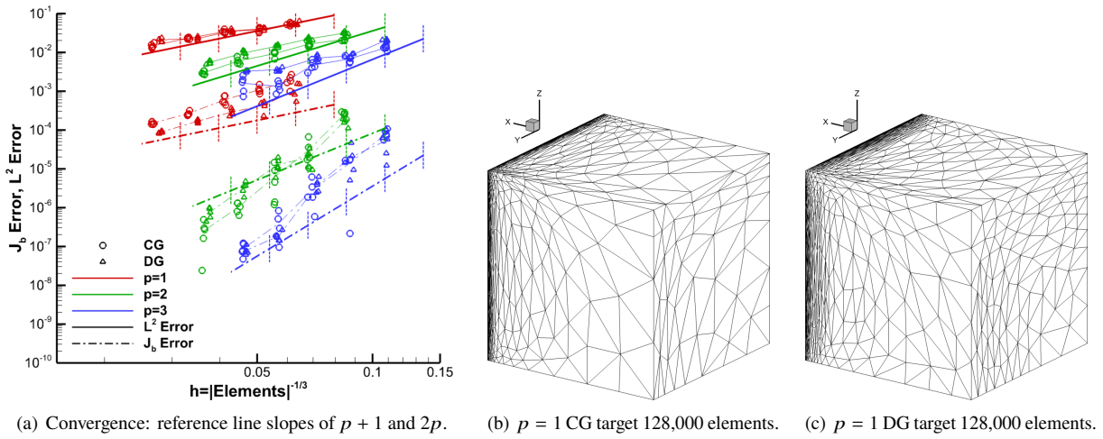
Fig. 65 TripleBL L^2 - and \mathcal{J}_b -error MOESS convergence and grids using FEFLO.A.
