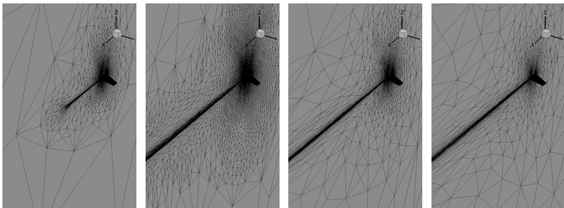
(e) FUN3D-SFE, L4, k -exact, Grad 10. (f) FUN3D-SFE, L2, k -exact, Grad 10. (g) FUN3D-SFE, L4, L2-proj, Grad 1.5. (h) FUN3D-SFE, L4, k -exact, Grad 1.5.
