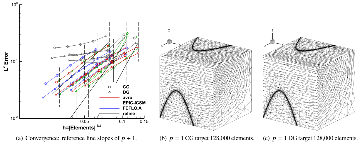
Fig. 13 sinatan3 L^2 -error MOESS convergence. Example meshes adapted with FEFLO.A.
