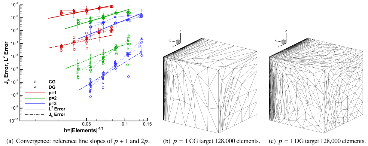
Fig. 20 TripleBL L^2 -error and \mathcal{J}_b -error MOESS convergence and grids using EPIC-ICSM.
