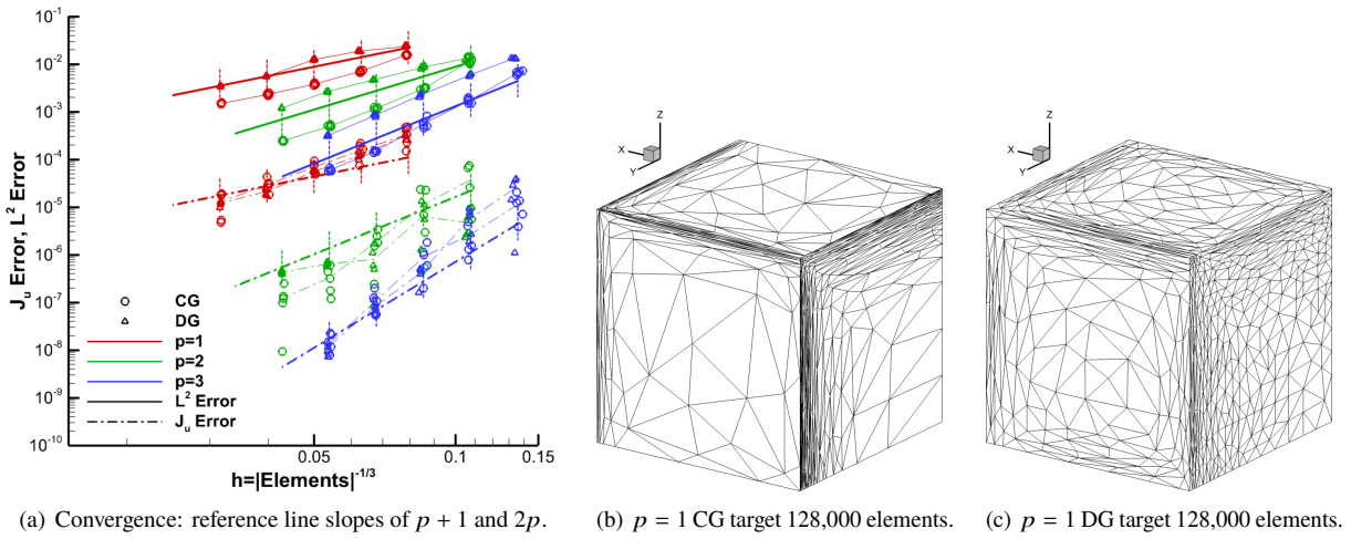
Fig. 18 TripleBL L^2 -error and J_u -error MOESS convergence and grids using EPIC-ICSM.
