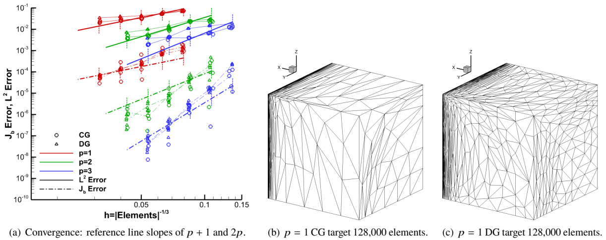
Fig. 66 TripleBL L^2 - and \mathcal{J}_b -error MOESS convergence and grids using EPIC-ICSM.
