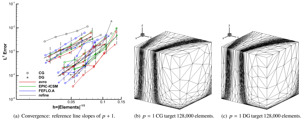
Fig. 9 \tanh 3 L^2 -error MOESS convergence. Example meshes adapted with FEFLO.A.
