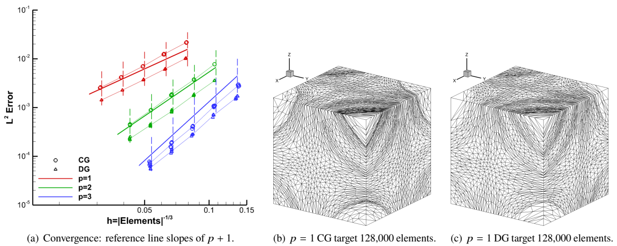
Fig. 36 \text{sinfun3} L^2 -error MOESS convergence and grids using EPIC-ICSM.
