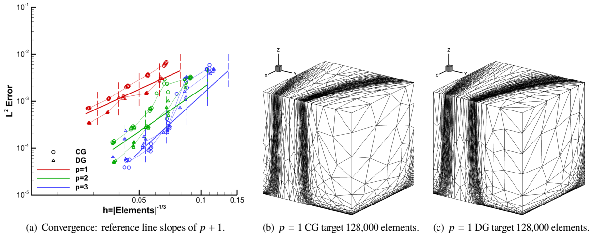
Fig. 44 \tanh 3 L^2 -error MOESS convergence and grids using FEFLO.A.
