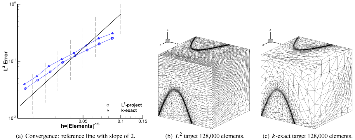
Fig. 48 sinatan3 L^2 -error multiscale metric convergence and grids using FEFLO.A .
