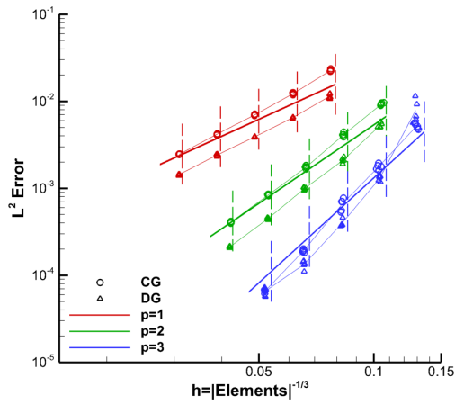
(a) Convergence: reference line slopes of p + 1 .
