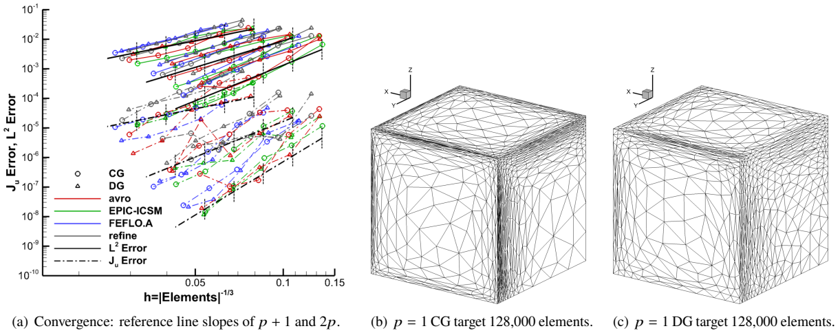
Fig. 17 TripleBL L^2 -error and J_u -error MOESS convergence. Example meshes adapted with FEFLO.A.
