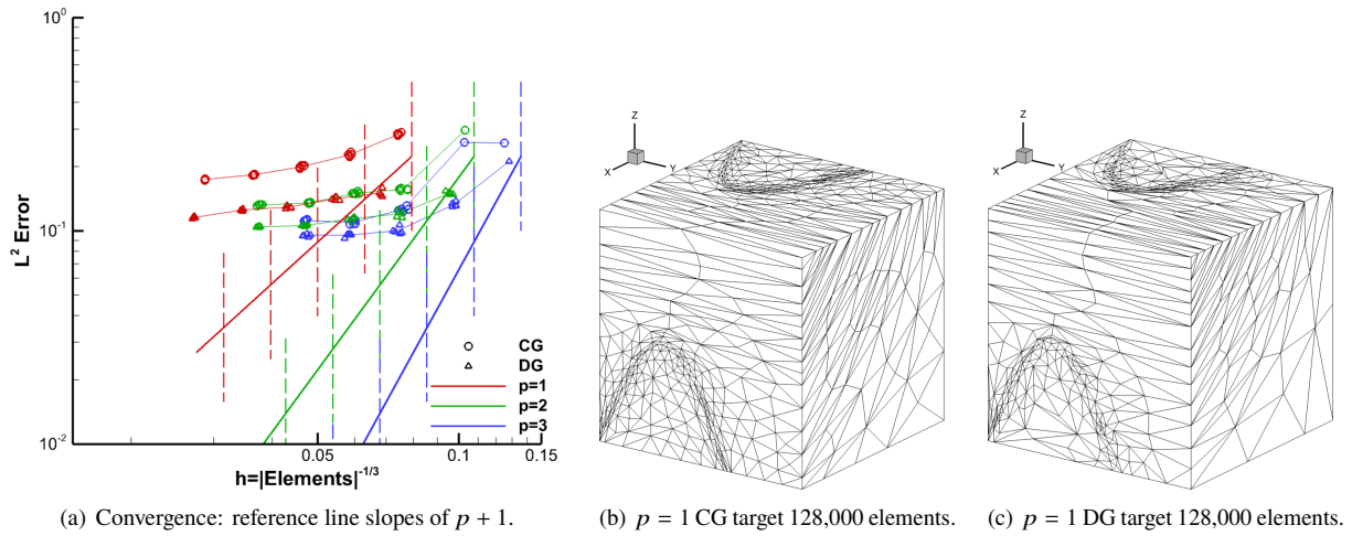
Fig. 52 sinatan3 L^2 -error MOESS convergence and grids using refine.
