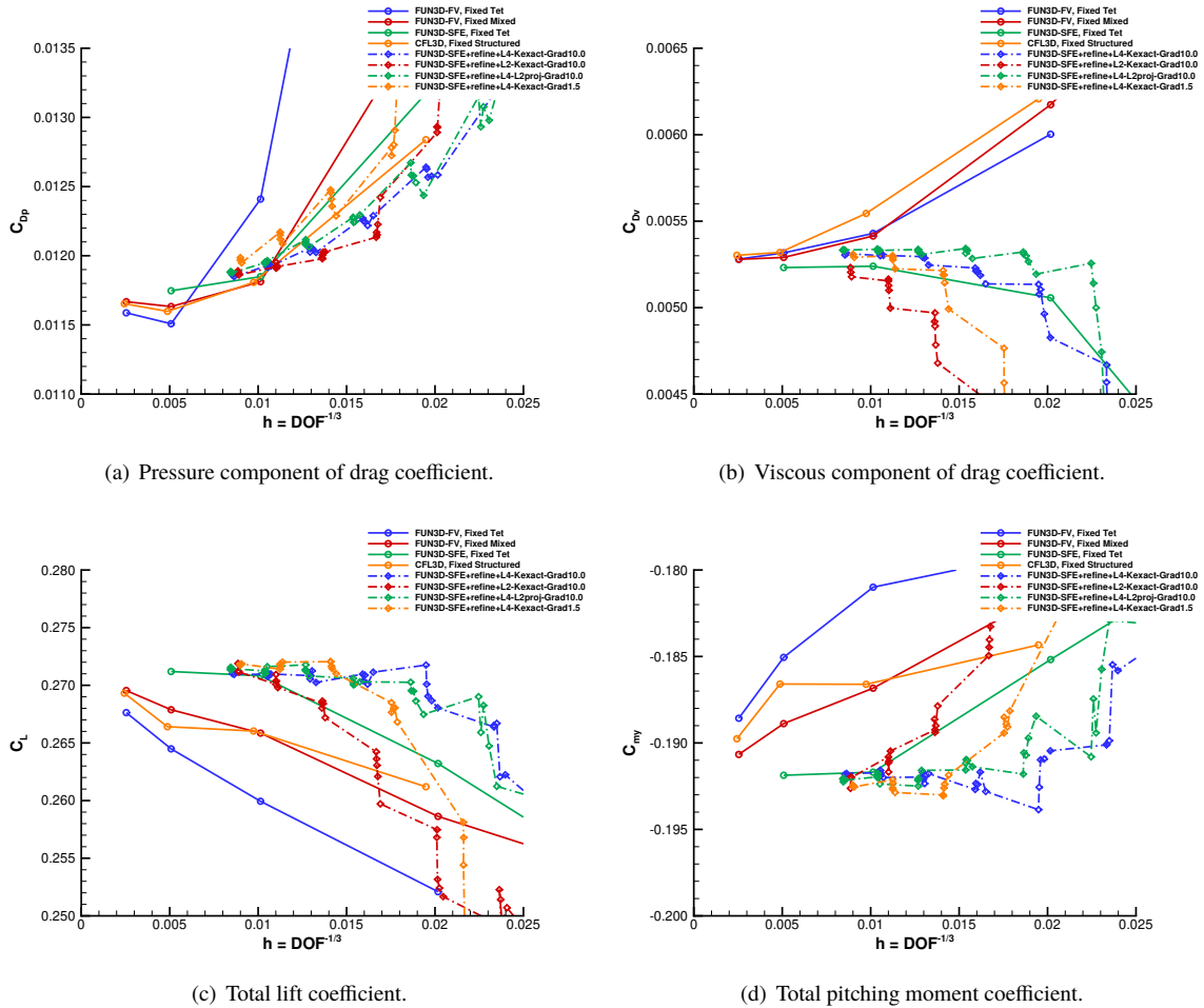
Fig. 71 ONERA M6 force and moment convergence, FUN3D-SFE+refine.
