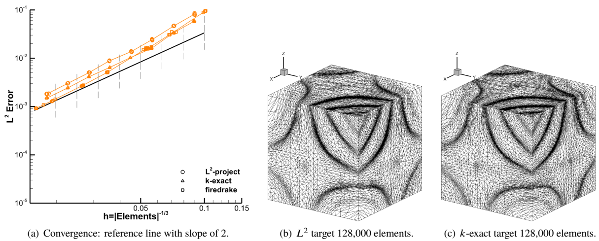
Fig. 33 sinfun3 L^2 -error multiscale metric convergence and grids using PRAGMaTic.
