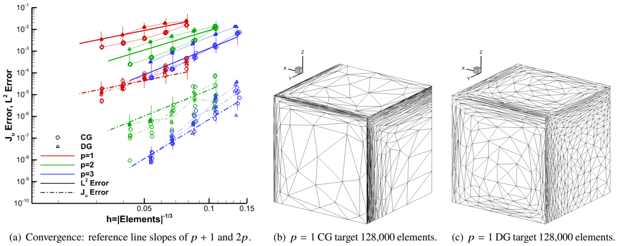
Fig. 62 TripleBL L^2 - and \mathcal{J}_u -error MOESS convergence and grids using EPIC-ICSM.
