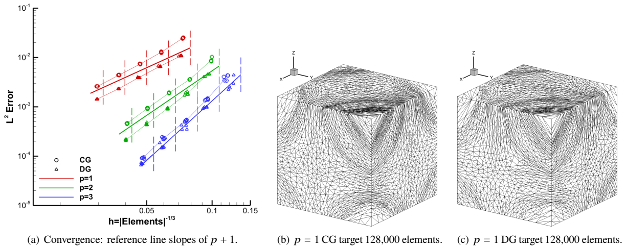
Fig. 34 \text{sinfun3} L^2 -error MOESS convergence and grids using refine.
