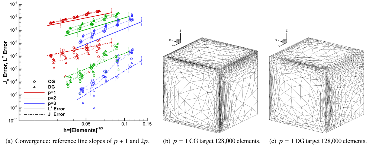
Fig. 61 TripleBL L^2 - and \mathcal{J}_u -error MOESS convergence and grids using FEFLO.A.
