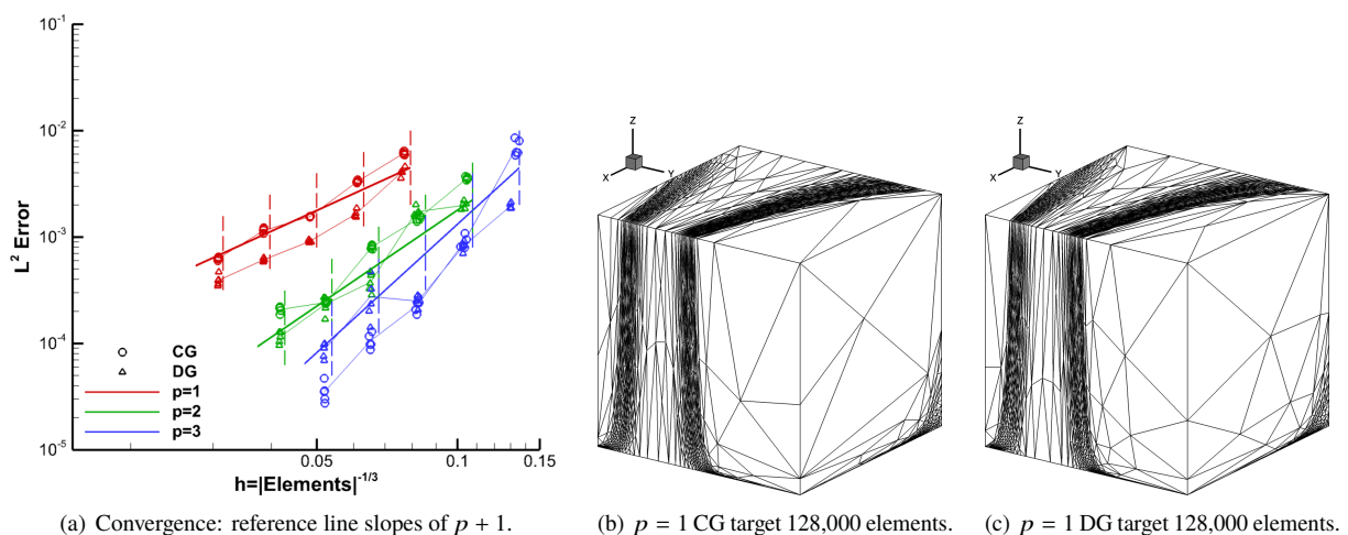
Fig. 46 tanh3 L^2 -error MOESS convergence and grids using avro.
